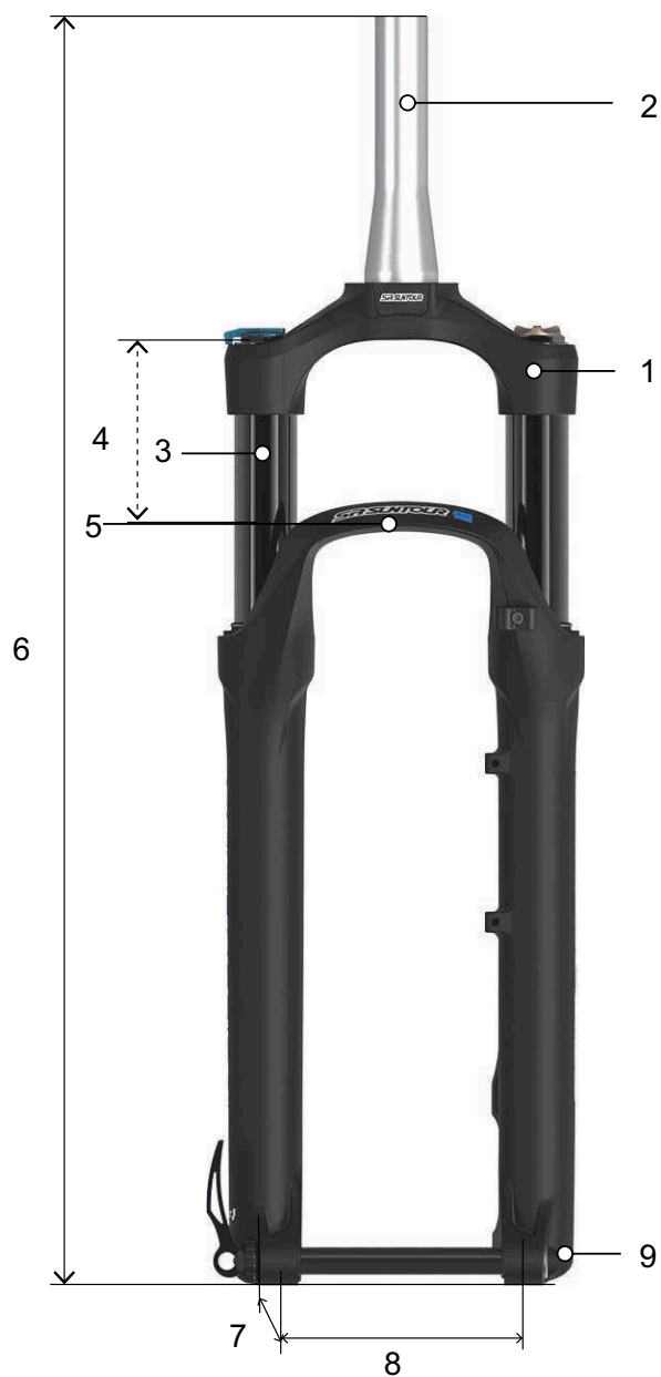
Slika 90: SR SUNTOUR, Mobie34, 2CRDS15LH1.507.5 ABS 27.5"
