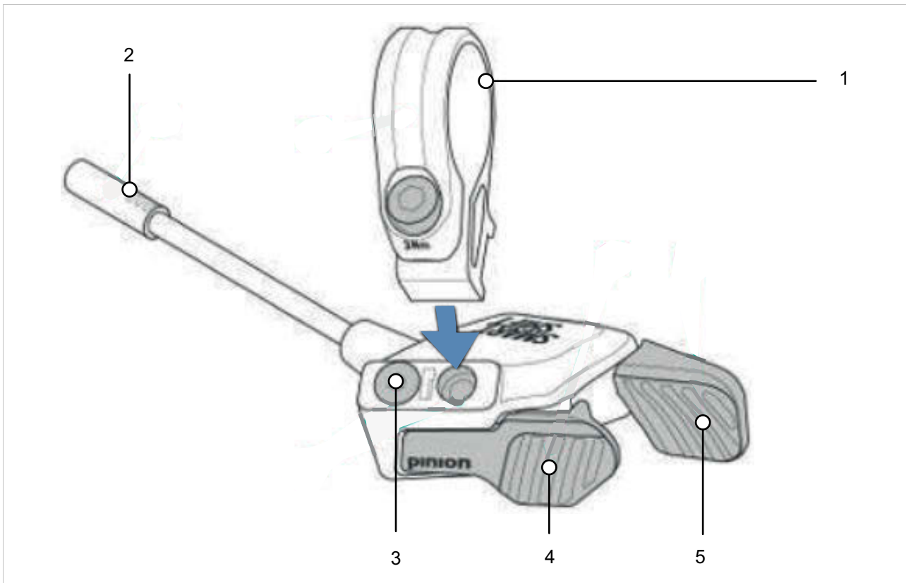
Illustration 62 : Structure Pinion E-Trigger TE1
